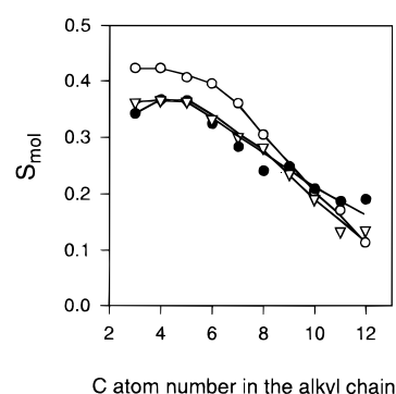
Figure 3. Time development of the profiles of the molecular order parameter. Keys: (O), 450–550 ps sample; (Δ), 1100–1200 ps sample; (●), 1500–1600 ps sample.
