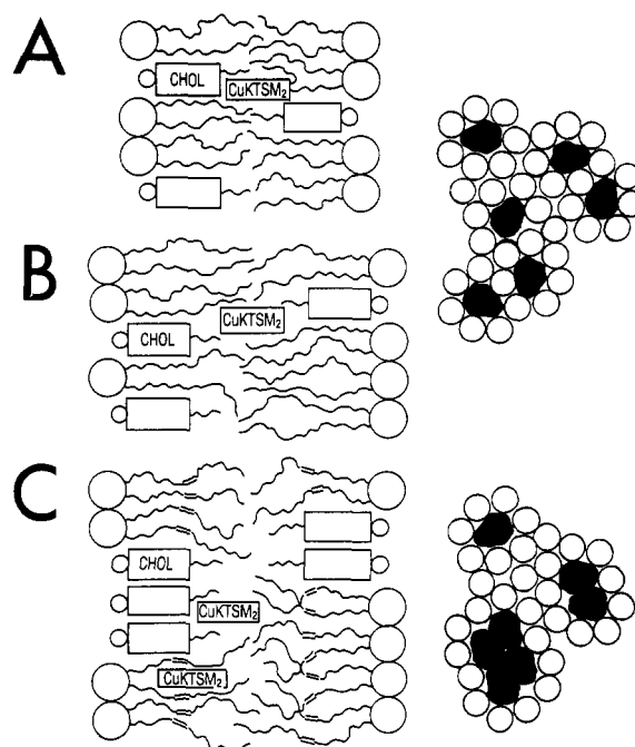
FIGURE 8: Schematic snapshot drawings of DMPC-cholesterol (A), DSPC-cholesterol (B), and DOPC-cholesterol (C) membranes with \text{CuKTSM}_2 . The drawings on the right side show the top-view models for saturated PC-cholesterol (top) and for unsaturated PC-cholesterol (bottom) membranes. The open circles represent the alkyl chains, and the solid structures [after Martin and Yeagle (1978)] indicate cholesterol molecules.
