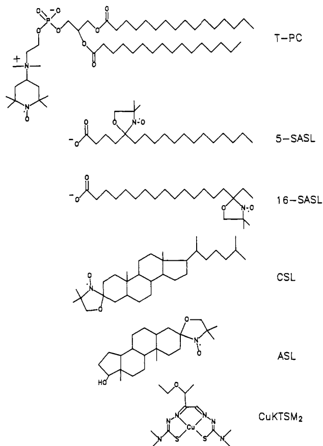
FIGURE 1: Structures of CuKTSM 2 , T-PC, 5-SASL, 16-SASL, CSL, ASL, and CuKTSM 2 .
