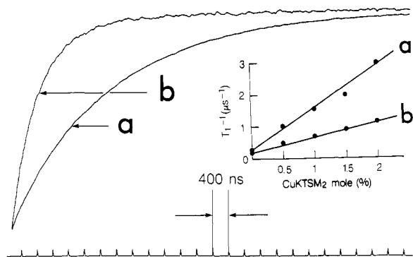
FIGURE 2: Typical saturation-recovery signal of 5-SASL in EYPC membranes containing 27.5 mol % cholesterol at 60 °C. Samples were equilibrated with nitrogen. (a) In the absence of CuKTSM 2 . T_1 = 2.61 \mu\text{s} . Conditions: pump power = 60 mW (microwave field = 1.2 G in the rotating frame); pump width = 9 \mu\text{s} . 4 \times 10^6 decays were accumulated during 2.7 min with 256 data points/decay. (b) In the presence of 0.5 mol % CuKTSM 2 . T_1 = 0.78 \mu\text{s} . Conditions were the same as above except that the pump width used was 5 \mu\text{s} . (Inset) T_1^{-1} of 5-SASL plotted as a function of the mole fraction of CuKTSM 2 in DMPC membranes measured at 45 °C (a) and 25 °C (b).
