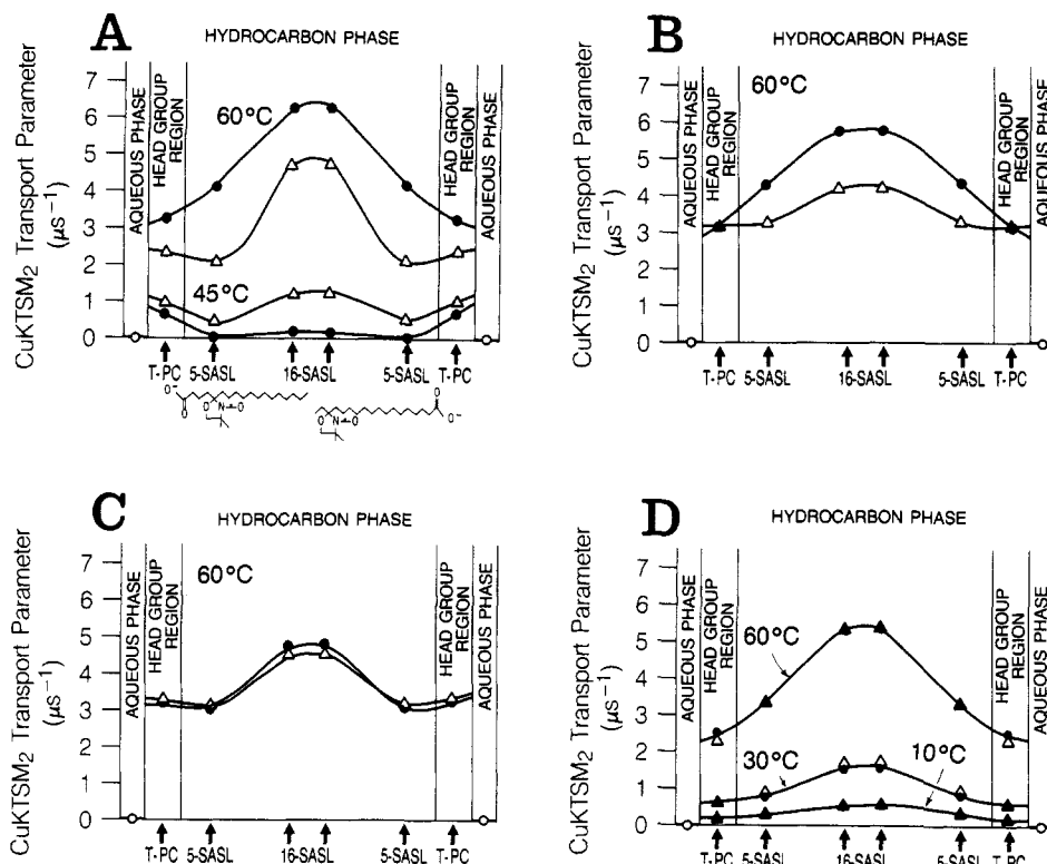
FIGURE 6: Effect of cholesterol on the W(\text{CuKTSM}_2) profiles across DSPC (A), DEPC (B), DOPC (C), and EYPC (D) membranes, estimated with T-PC, 5-SASL, 16-SASL, and Tempon. Approximate locations of the nitroxide are indicated by arrows as well as by the drawings of SASL. Closed and open keys indicate the absence and presence of 27.5 mol % cholesterol, respectively.
